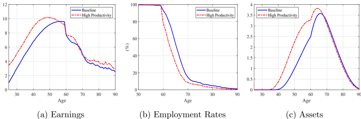
Figure 19: Productivity Growth
